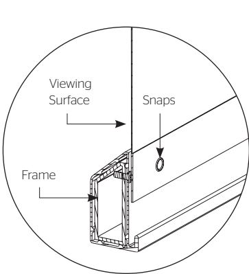
Viewing Surface & Frame Detail
